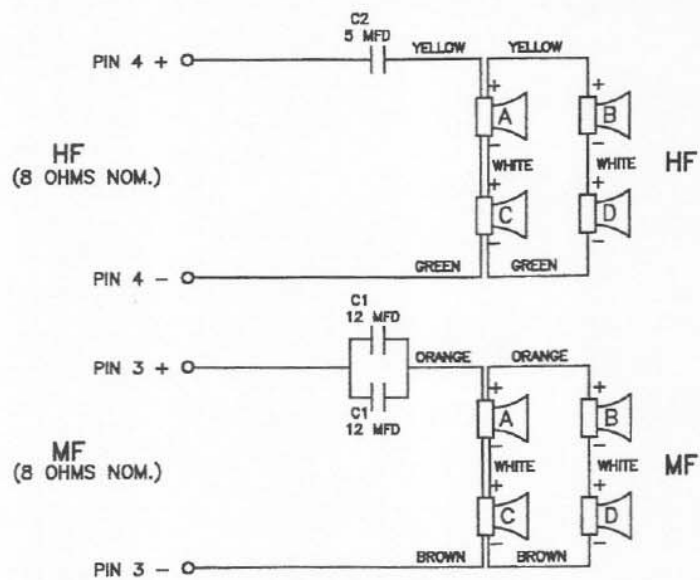
WIRING DIAGRAM
